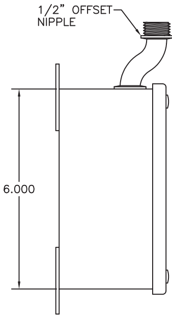
Figure 1: Mechanical Dimensions (in.) Unit shown is a three-phase wye
