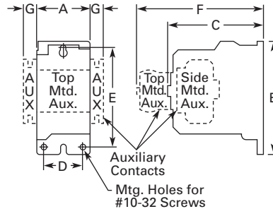
Sizes 0-2, Two- and Three-Pole
