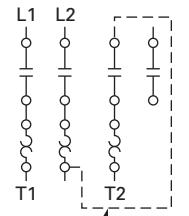
Field Conversion to Single-Phase, Add Dotted Connections
